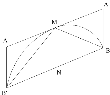
Figure 1. A Parabolic Segment and its Archimedean Triangle
