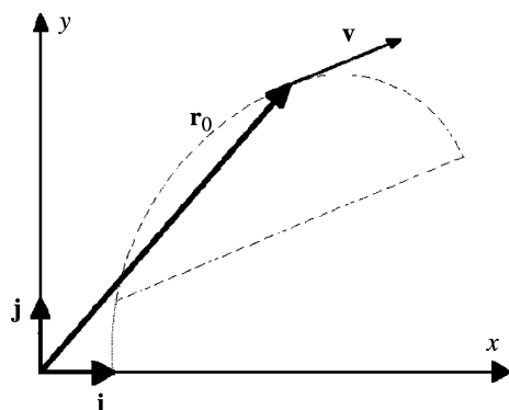
Figure 2. Initial Conditions for Parabolic Flight
