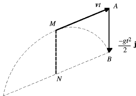
Figure 3. Trajectory from M to B .
