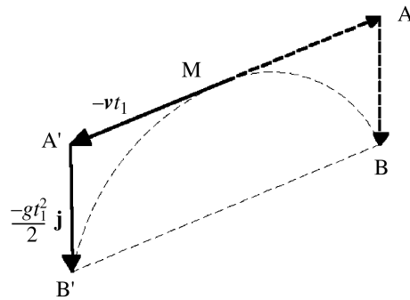
Figure 4. Trajectory from M to B'
