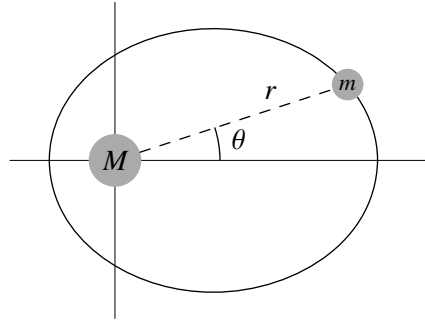
Figure 1 – Elliptical orbit
